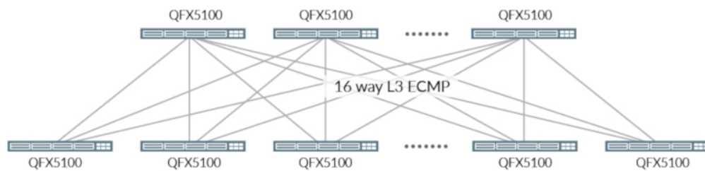
Figure 4: Larger scale data center with Layer 3 to the access
